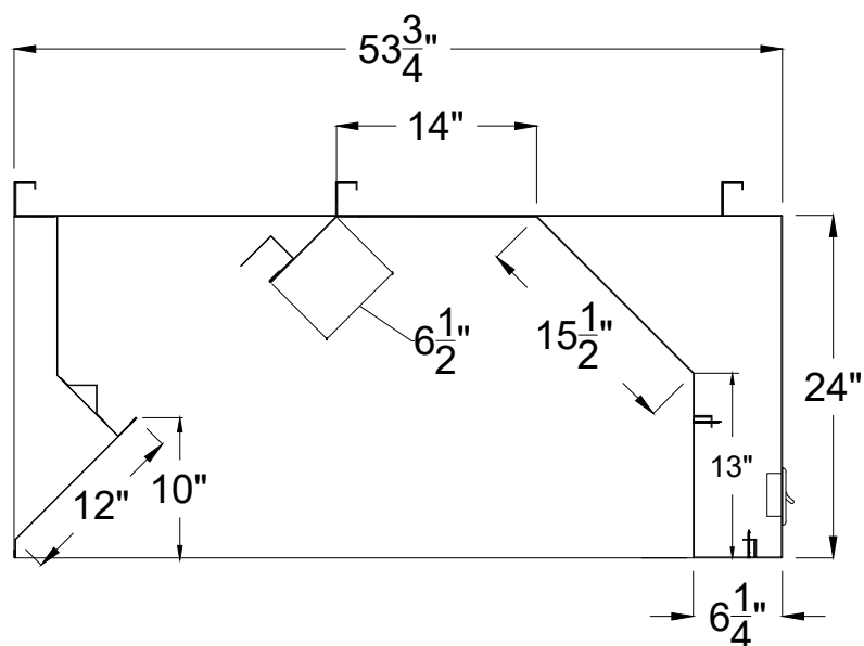
Section View A-A: Wall Canopy Hood with Make-up Air
